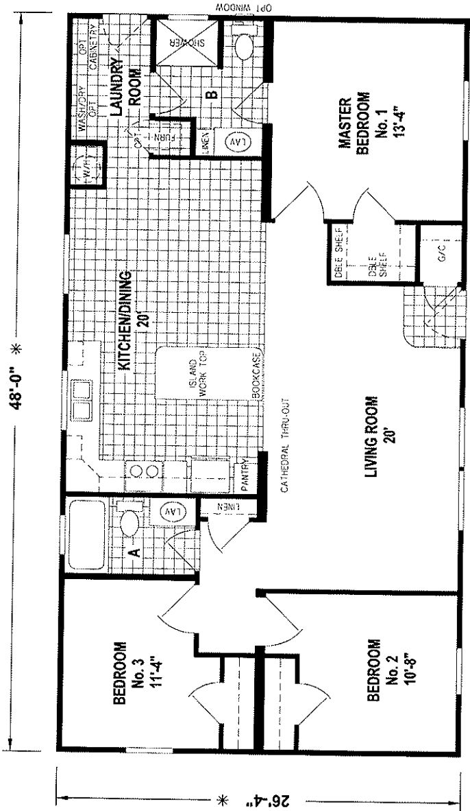
A205CTV/4828 (1,264 SQ. FT.) 3BEDROOM - 2BATHS - CATHEDRAL THRU-OUT
